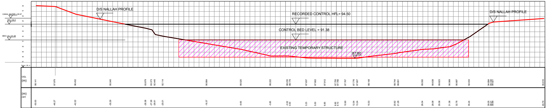
SECTION ALONG SYPHON CONTROL SECTION (WITH EXISTING TEMPORARY STRUCTURE) SECTION CH. + 240
