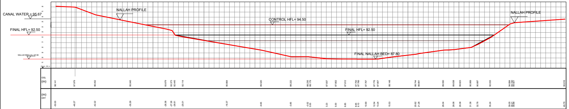
SECTION ALONG SYPHON SECTION WITH EQUIVALENT DISCHARGE (AFTER REMOVAL OF TEMPORARY STRUCTURE) SECTION CH. + 240
